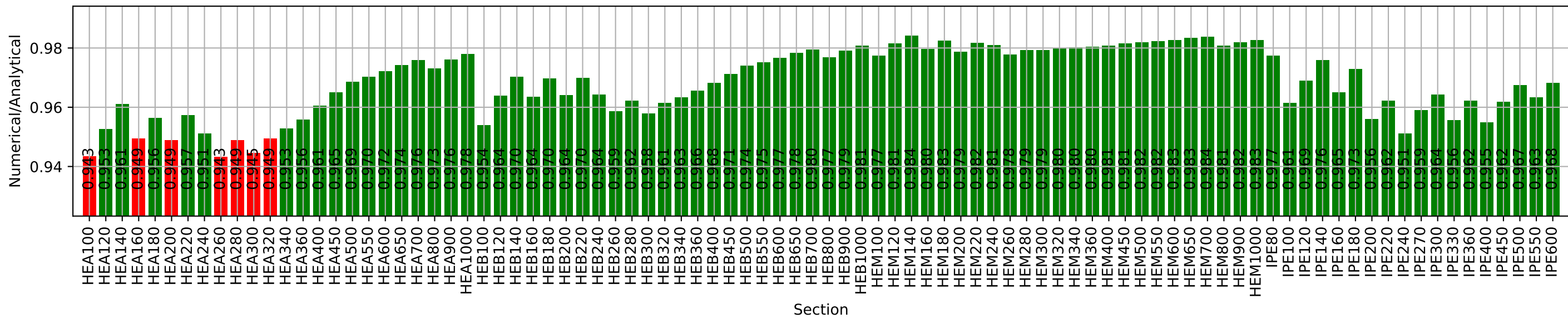
EU Strong Axis Moment of Inertia
