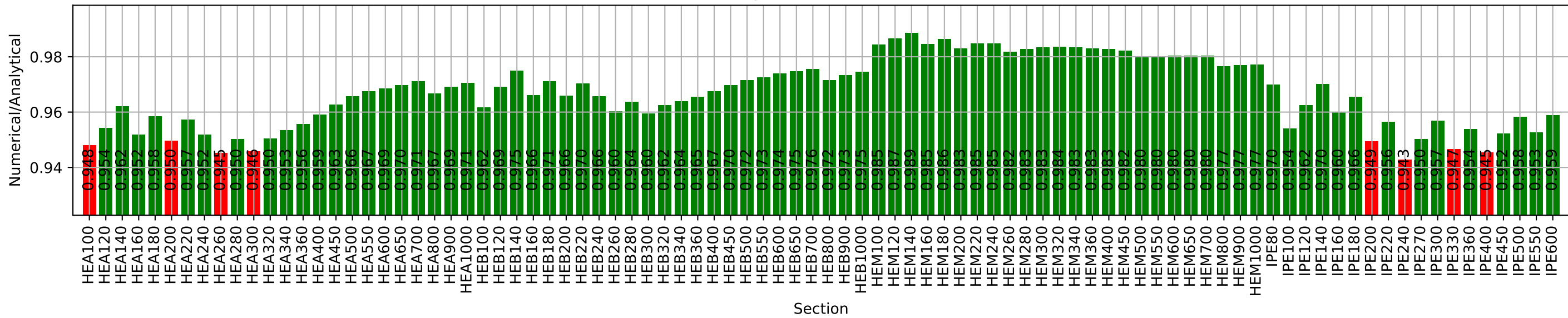
EU Weak Axis Moment of Inertia
